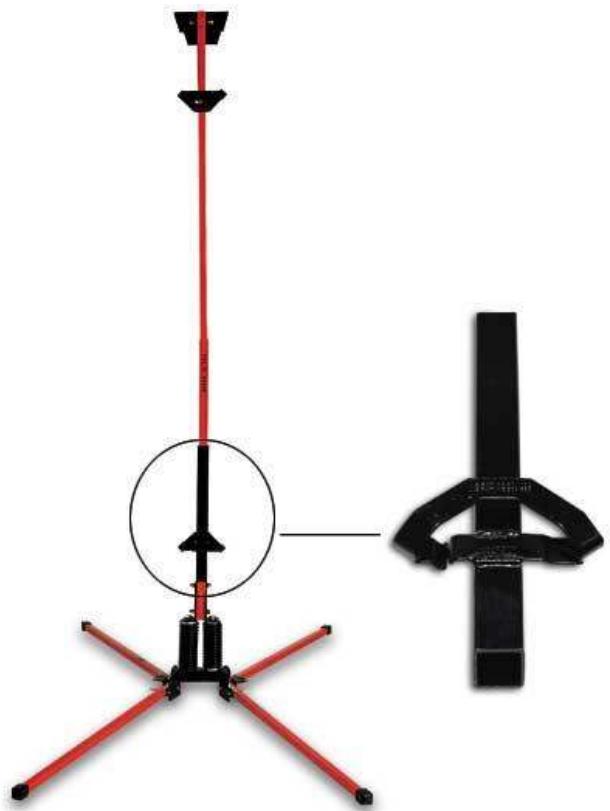
Little Buster Sign Stand with Safe Sleeve-350 Bracket for use with .080 aluminum signs
